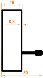
Platin Tekli Kasa Profil Platin Single Case Profile
