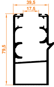
Üstten Fitilli Büyük Oluklu Kasa Large Corrugated Case with Top Wick
